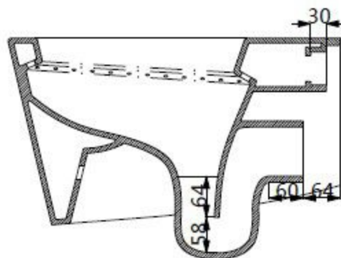
SECTION_VIEW A-A
